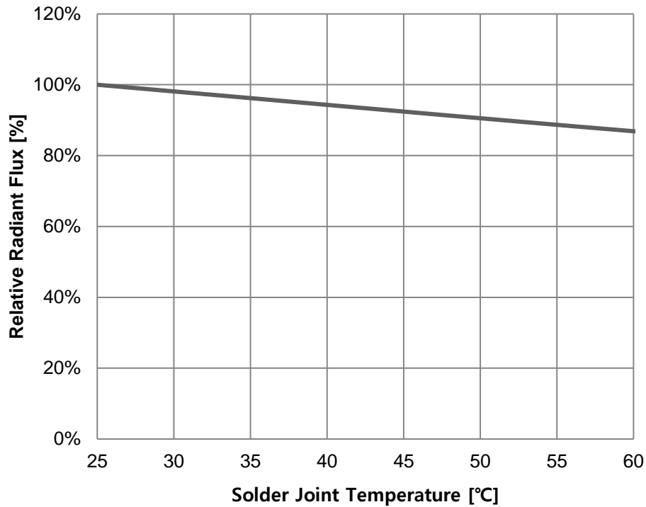
Fig 5. Surface Temperature vs. Relative Radiant Flux, I_F=600\text{mA}
